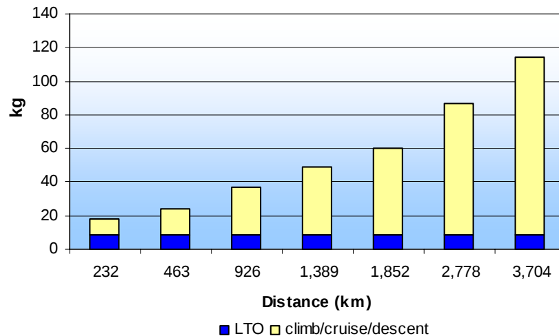
Figure 13 : Total \text{NO}_x emissions from aircraft (B737 400) related to flight phase and distance
