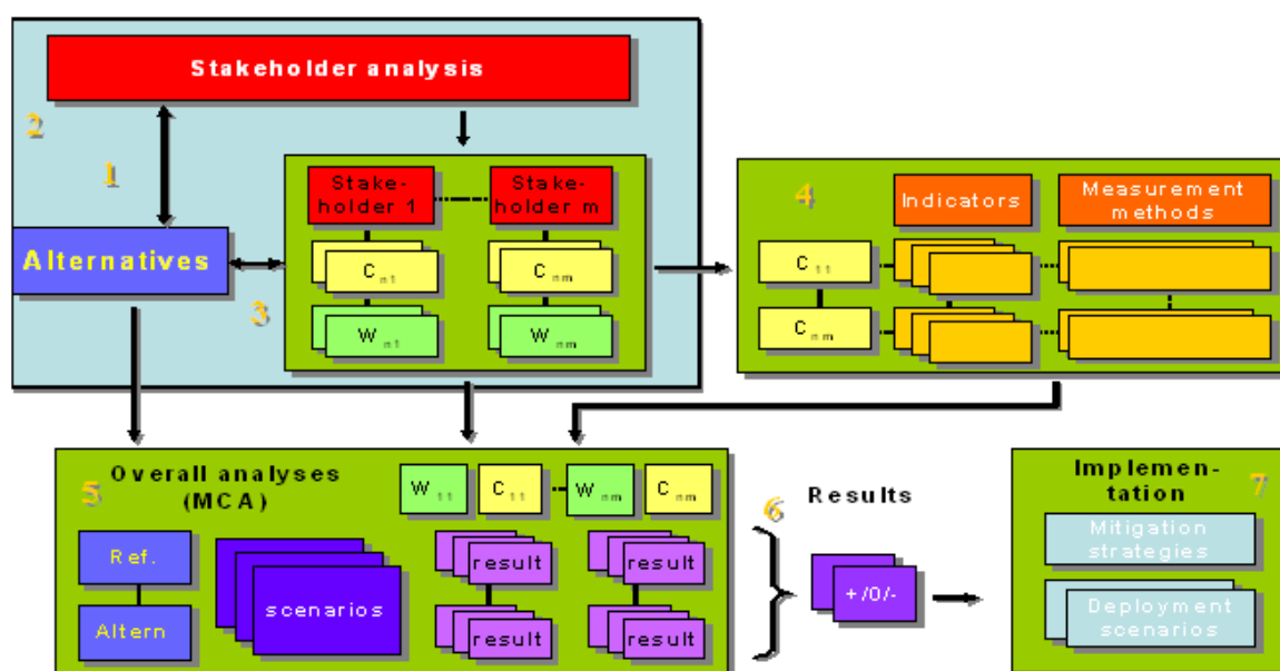
Figure 49 : MAMCA scheme
